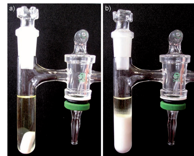
Figure 1. The reaction of isovaleraldehyde with 2-naphthyl N -Boc-imine in the presence of ( S )-proline (20 mol%; Table 1, entry 6) in CH 3 CN. a) Homogenous reaction mixture after mixing all components. b) Reaction mixture after completion of the reaction (10 h).
